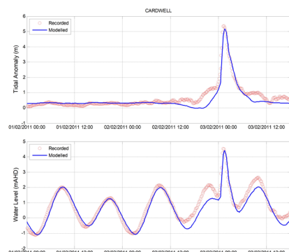
Storm Tide Calibration
