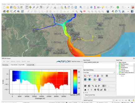
Complex estuary easily resolved with flexible mesh
