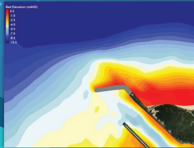
Breakwater Design - Siltation
